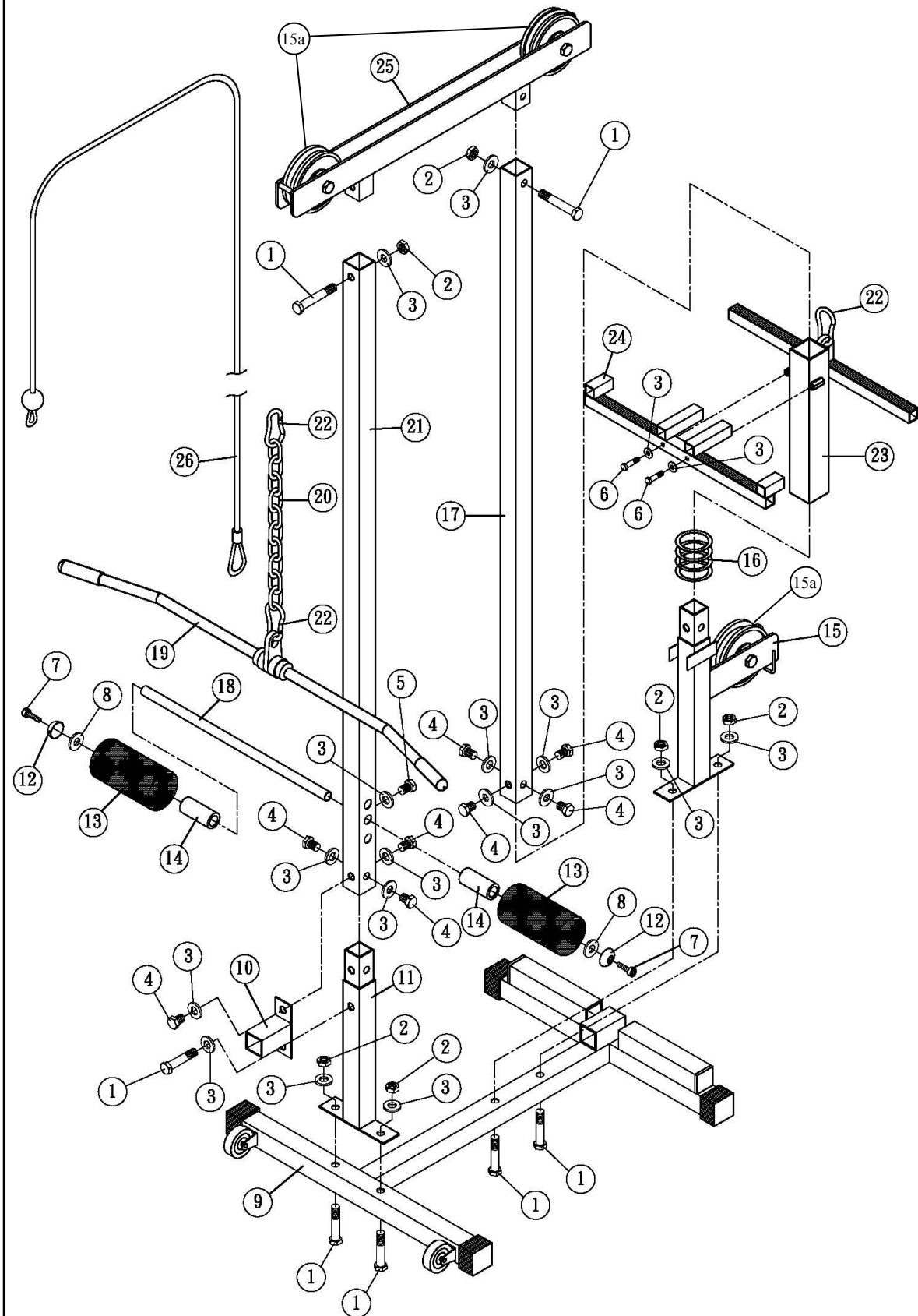
Exploded View—Ironmaster Cable Tower
